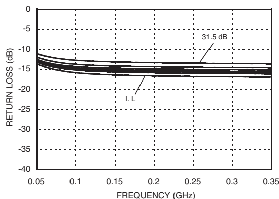
Output Return Loss [3]
