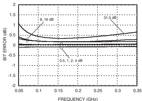
Bit Error vs. Frequency [3]
